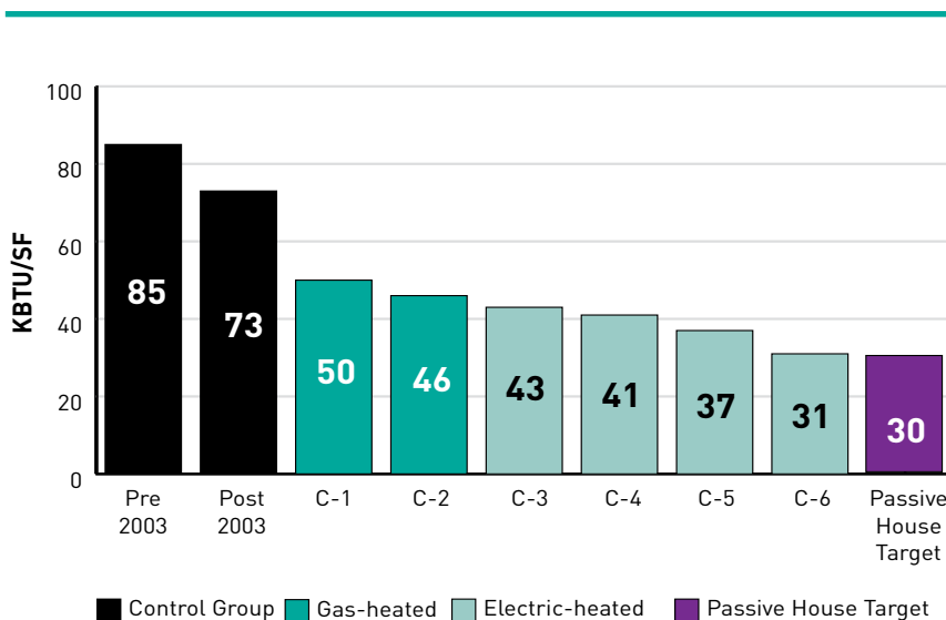
Figure B. Looking at Energy Use Intensity (EUI), the Passive House case study buildings consume 32-58% less energy than the buildings in the post-2003, conventionally-built control group. 5
